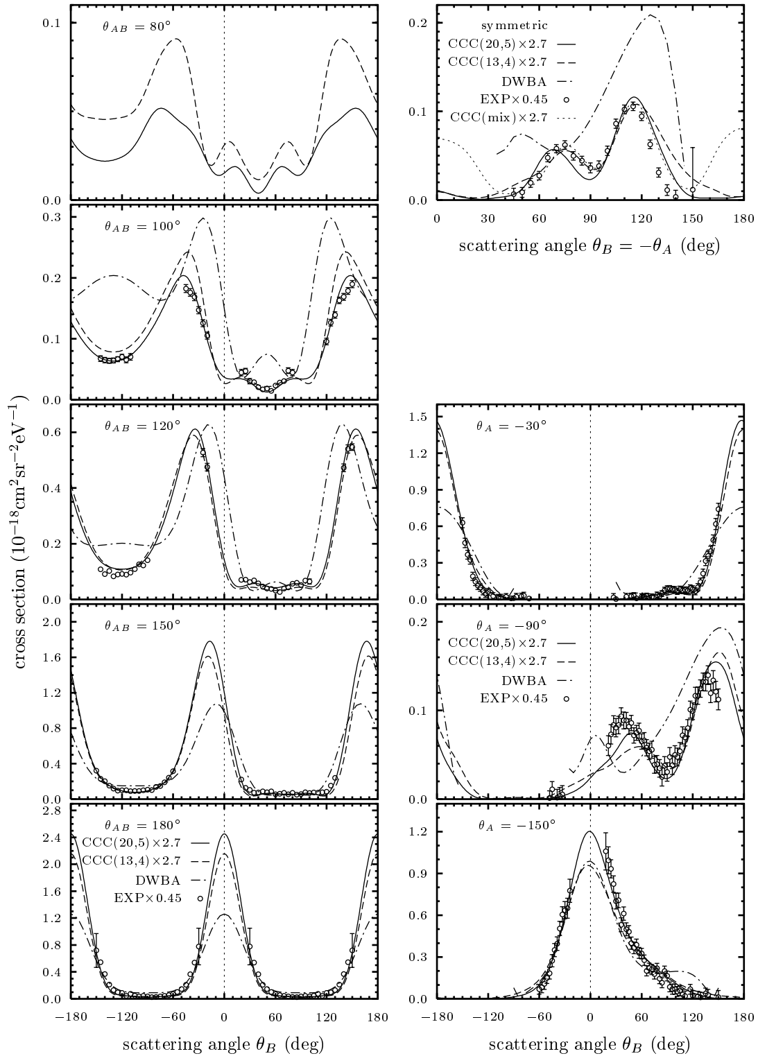
Figure 2. The coplanar triply differential cross sections, in the indicated geometries, for electron-impact ionization of atomic hydrogen with 1 eV outgoing electrons. Absolute experiment of Röder et al (1997b) has been scaled by a factor of 0.45 for best visual fit to the rescaled CCC data, see text. The DWBA calculations are due to Jones et al (1992).
